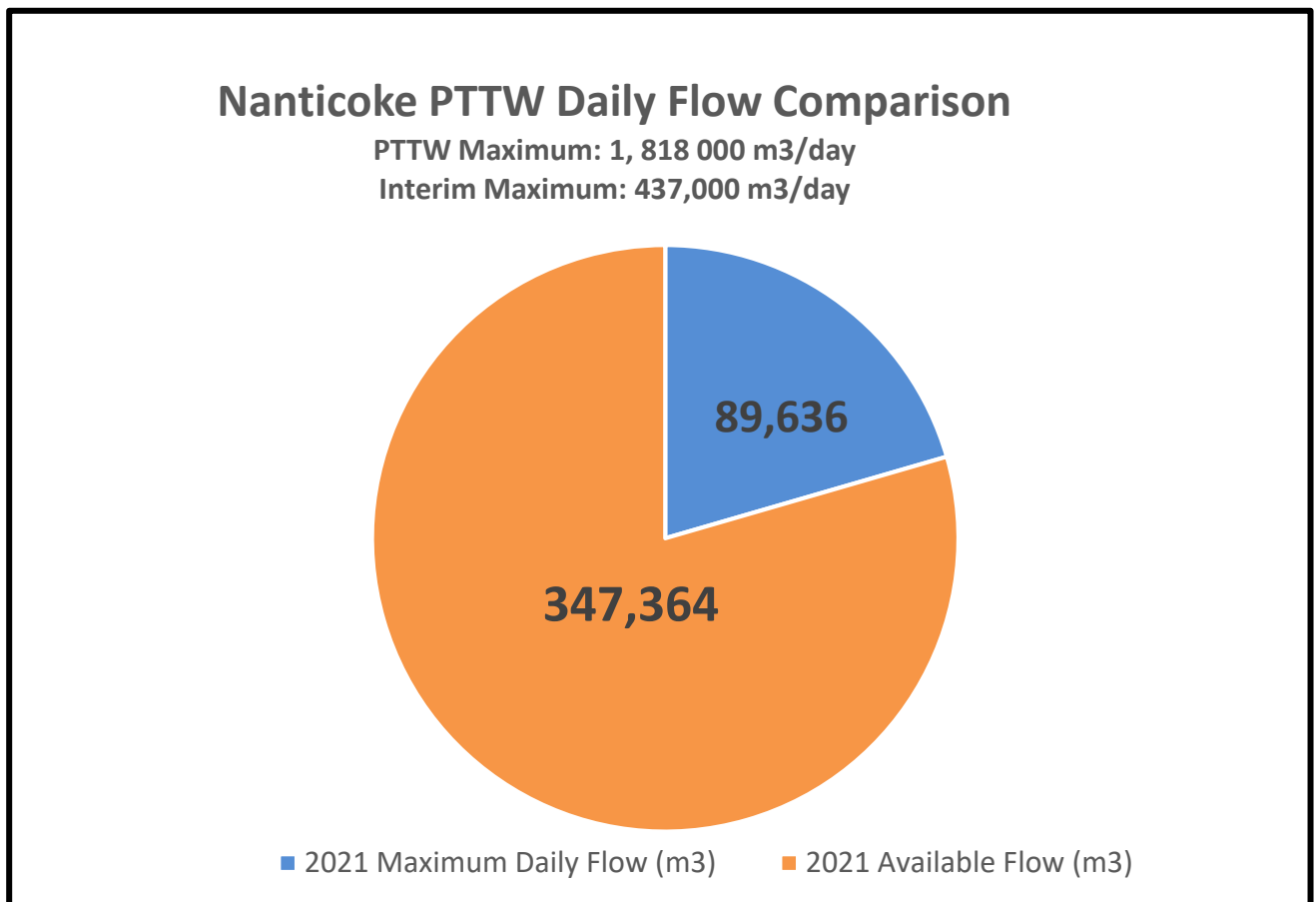
Figure 3: Nanticoke Permit To Take Water Flow Comparison
